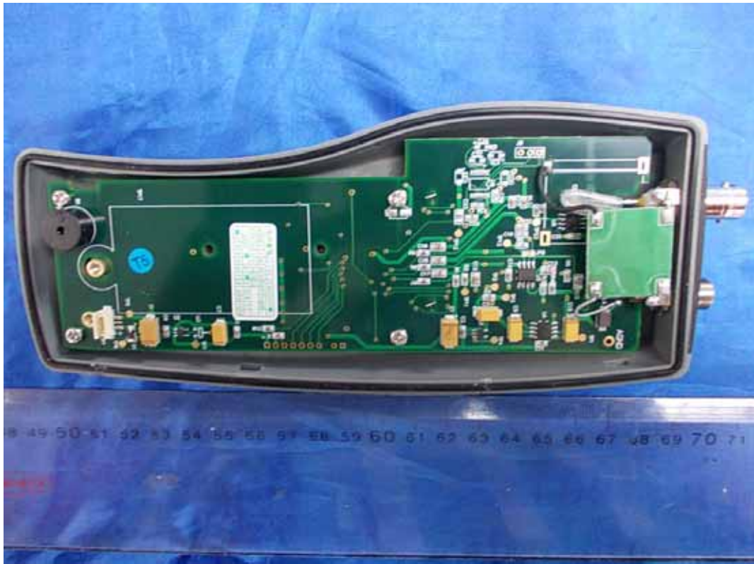
FIGURE 7 PORTABLE PH, MV AND TEMPERATURE INSTRUMENT (M/N: PH100A) MAIN BOARD (COMPONENT SIDE)
