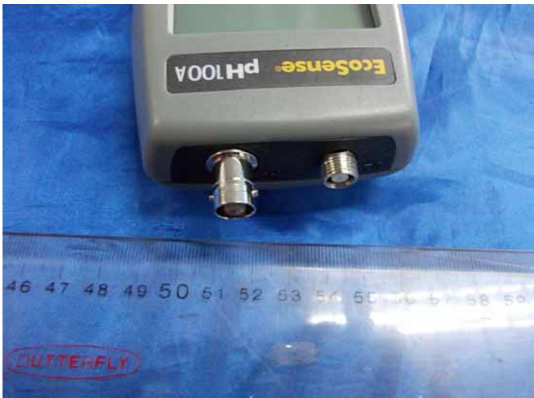
FIGURE 5 PORTABLE pH, mV AND TEMPERATURE INSTRUMENT (M/N: pH100A) PORTS VIEW
